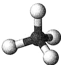
Tetrahedral
