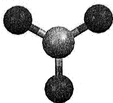
Trigonal Planar
