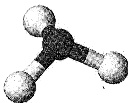
Trigonal Pyramidal
